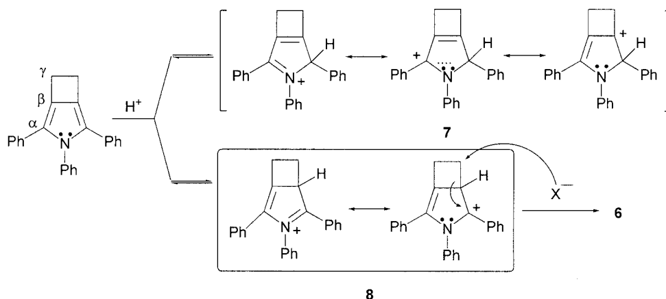
Scheme 2. Mechanism of ring-opening of 5a by electrophiles
