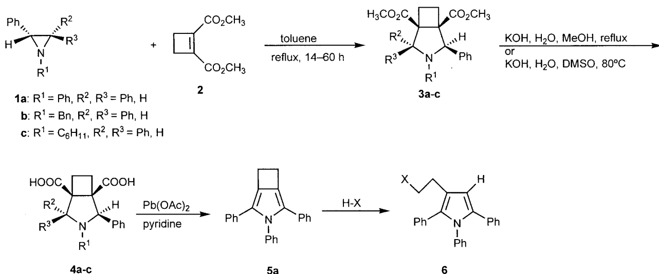
Scheme 1. Synthesis of 5a and ring-opening by electrophiles
