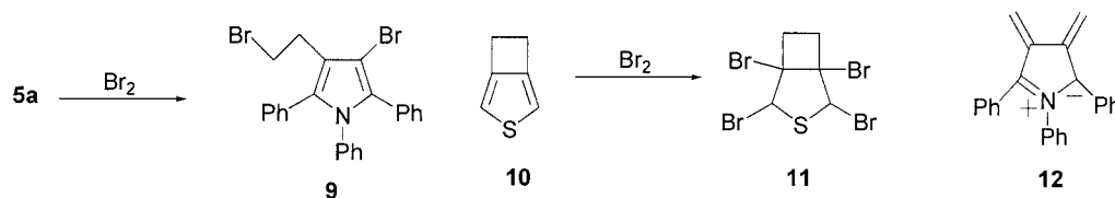
Scheme 3. Reaction of bromine with 5a compared with 10
