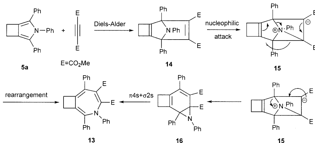
Scheme 4. Plausible mechanism for the formation of the azepine 13 on treatment of 5a with DMAD
